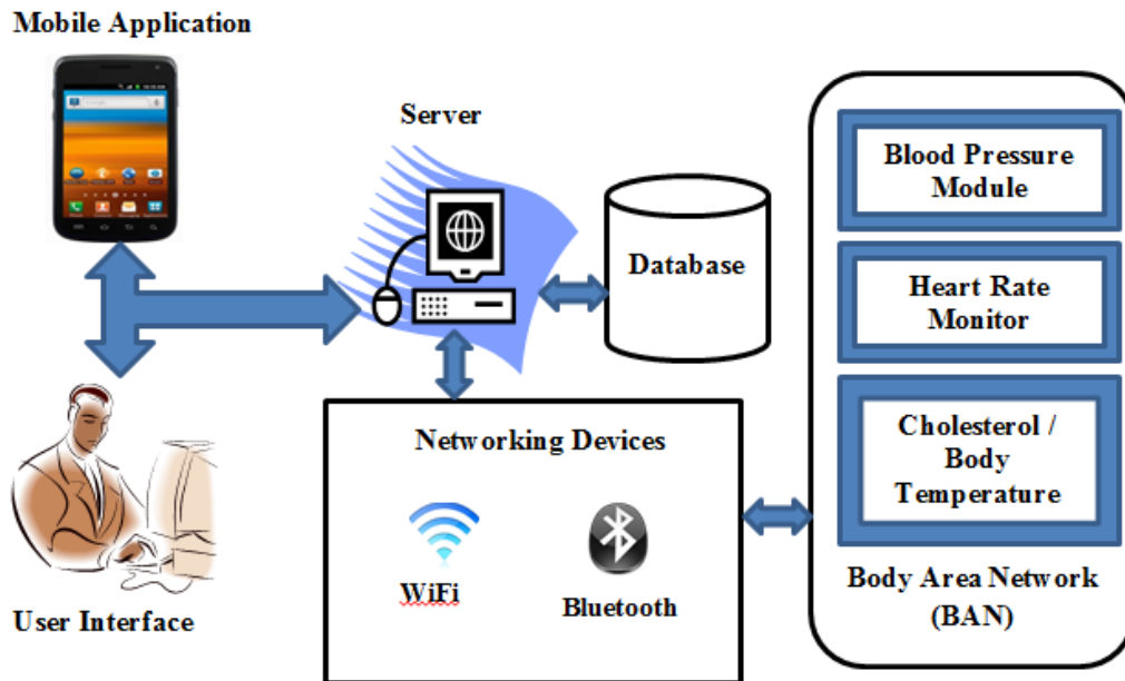
Figure.1. Architecture of Patient Health Monitoring System (PHMS)
