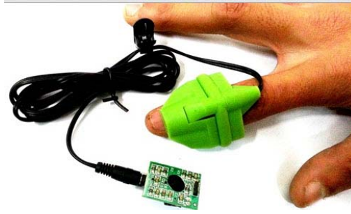
Figure.2. Heartbeat sensor with 8051 Microcontroller [3]
